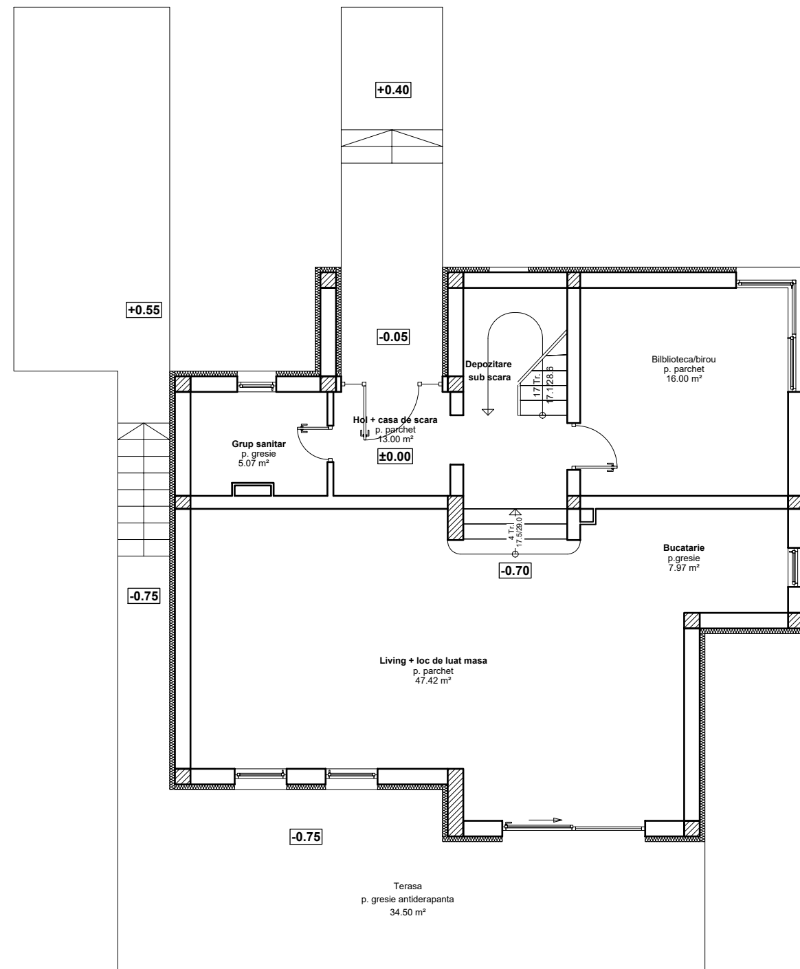
Plan parter 112.17 mp
